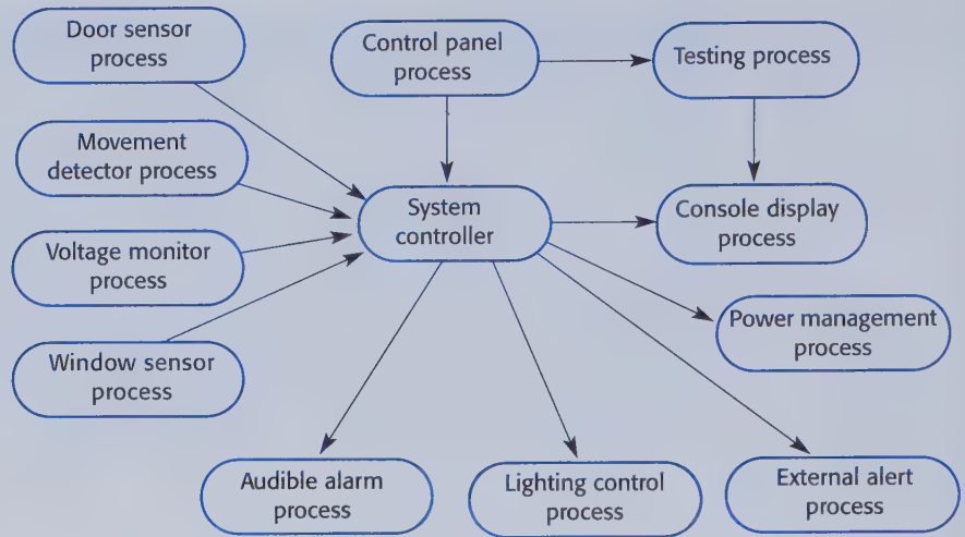
Figure 21.8 The process structure of a burglar alarm system
