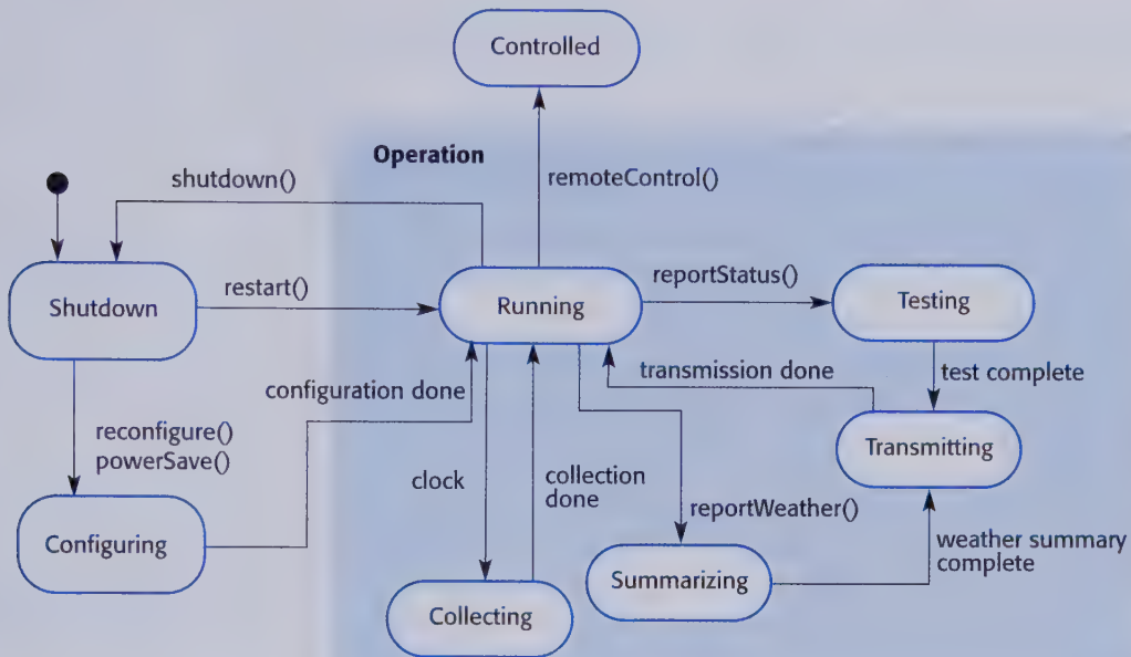
Figure 7.8 Weather station state diagram
