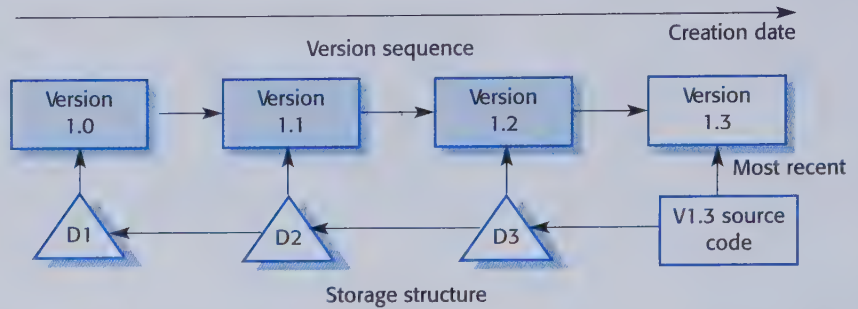
Figure 25.9 Storage management using deltas
