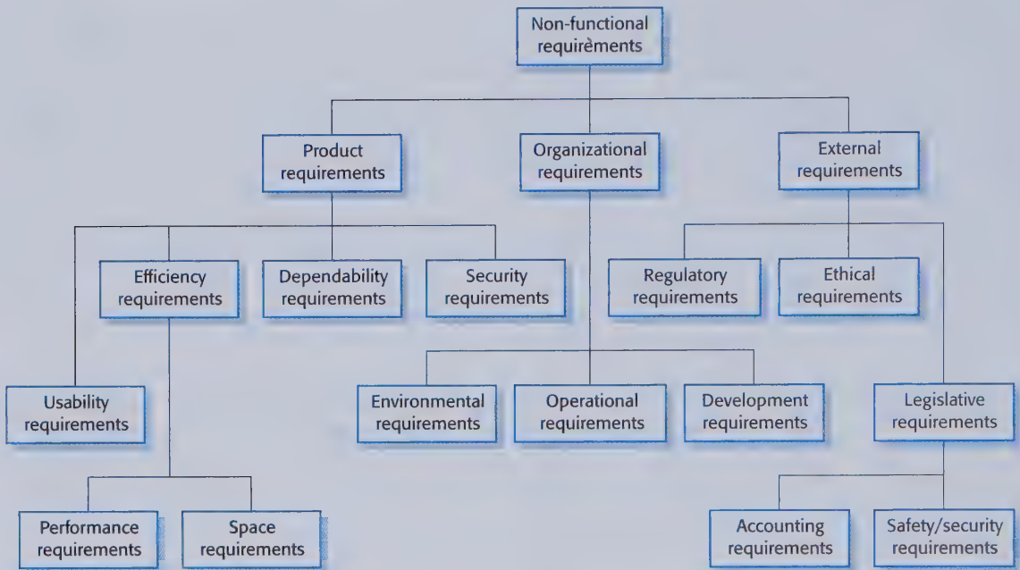
Figure 4.3 Types of non-functional requirements
